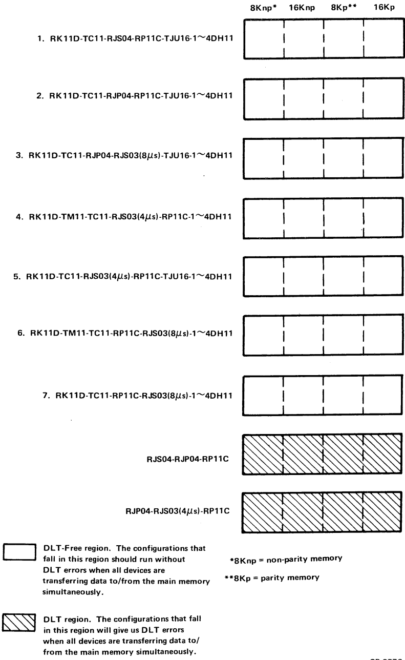
Figure 2-24 DLT Configurations
