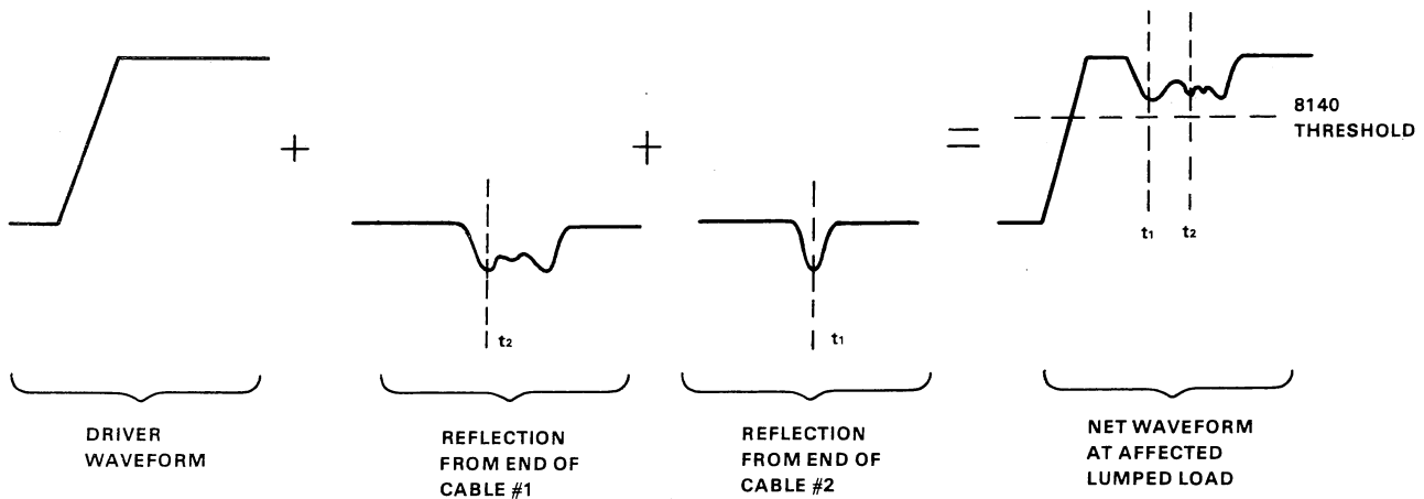
Figure 2-18 Implementation of Rule No. 5 (Waveform Example)
