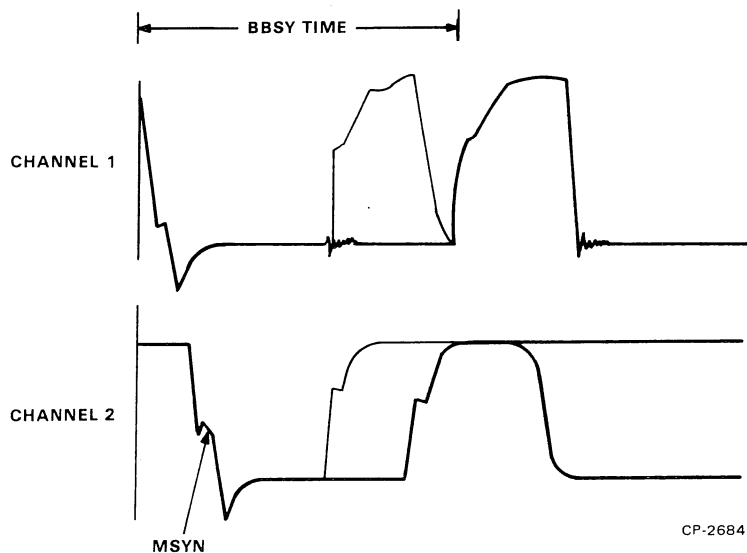
Figure 2-22 Single-Cycle Transaction
