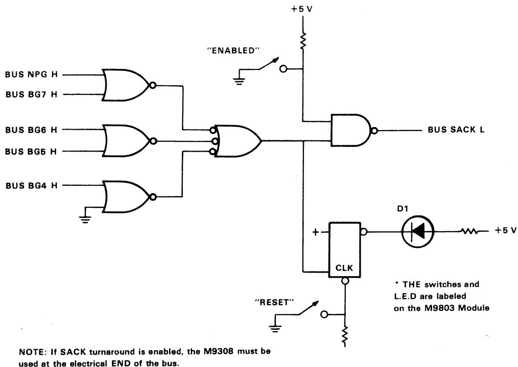
Figure 4-17 M9308 SACK Turnaround Logic
